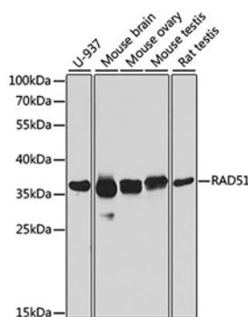
Fig. 1. Western blot analysis of extracts of various cell lines, using RAD51 antibody at 1:1000 dilution. Secondary antibody: HRP-labeled Goat Anti-Rabbit IgG(H+L) (A0208) at 1:1000 dilution. Lysates/proteins: 25 \mu g per lane. Blocking buffer: QuickBlock TM Blocking Buffer (P0231). Detection: BeyoECL Star (P0018A). Exposure time:1s.
